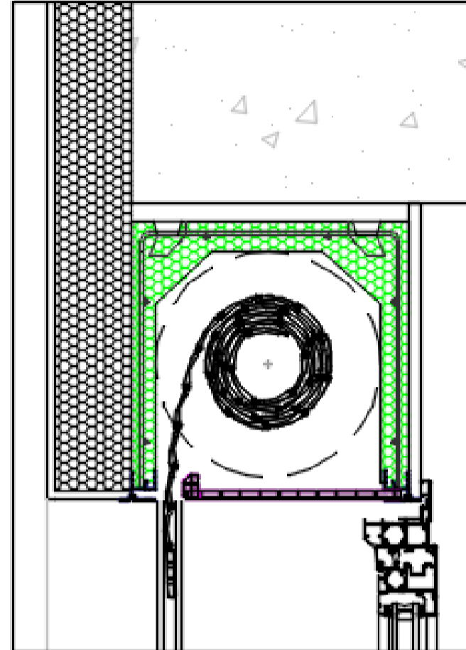
SATE
